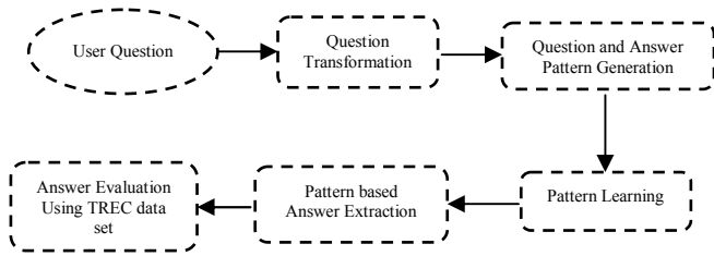
Figure 1. Pattern based answer extraction.
